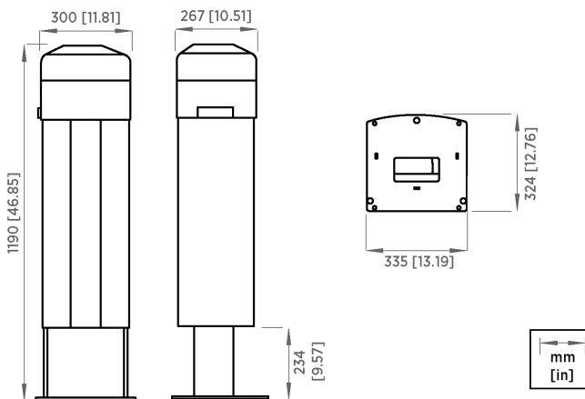
Ceilometer CL31 dimensions
